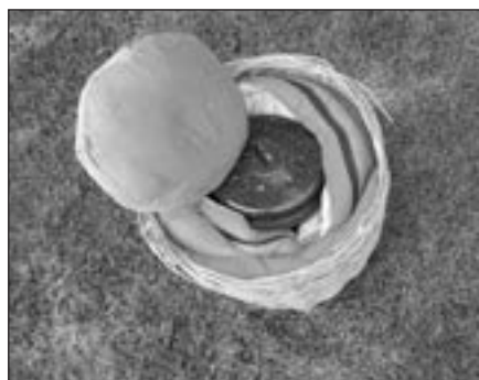
Figure 1 Retained heat cooker (photo: Darwin Curtis)
