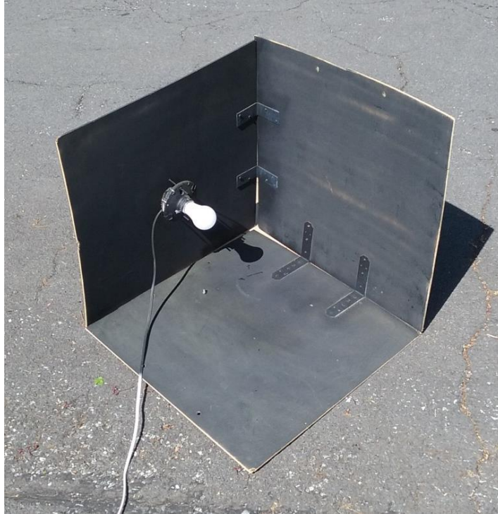
Figure 3. Rig for measuring bare bulb directivity.
